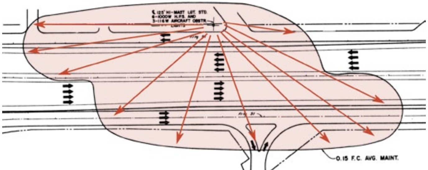
The Z-pattern high mast configuration: The first generation of high mast lighting on linear sections of Houston's freeways, installed from 1979 to the early 1990s, featured the Z-pattern lighting configuration. The Z-pattern was designed to provide light from above and behind the driver so the driver would never look directly into a floodlight. (Graphic: Z-Pattern High Mast Freeway Illumination 115 )
